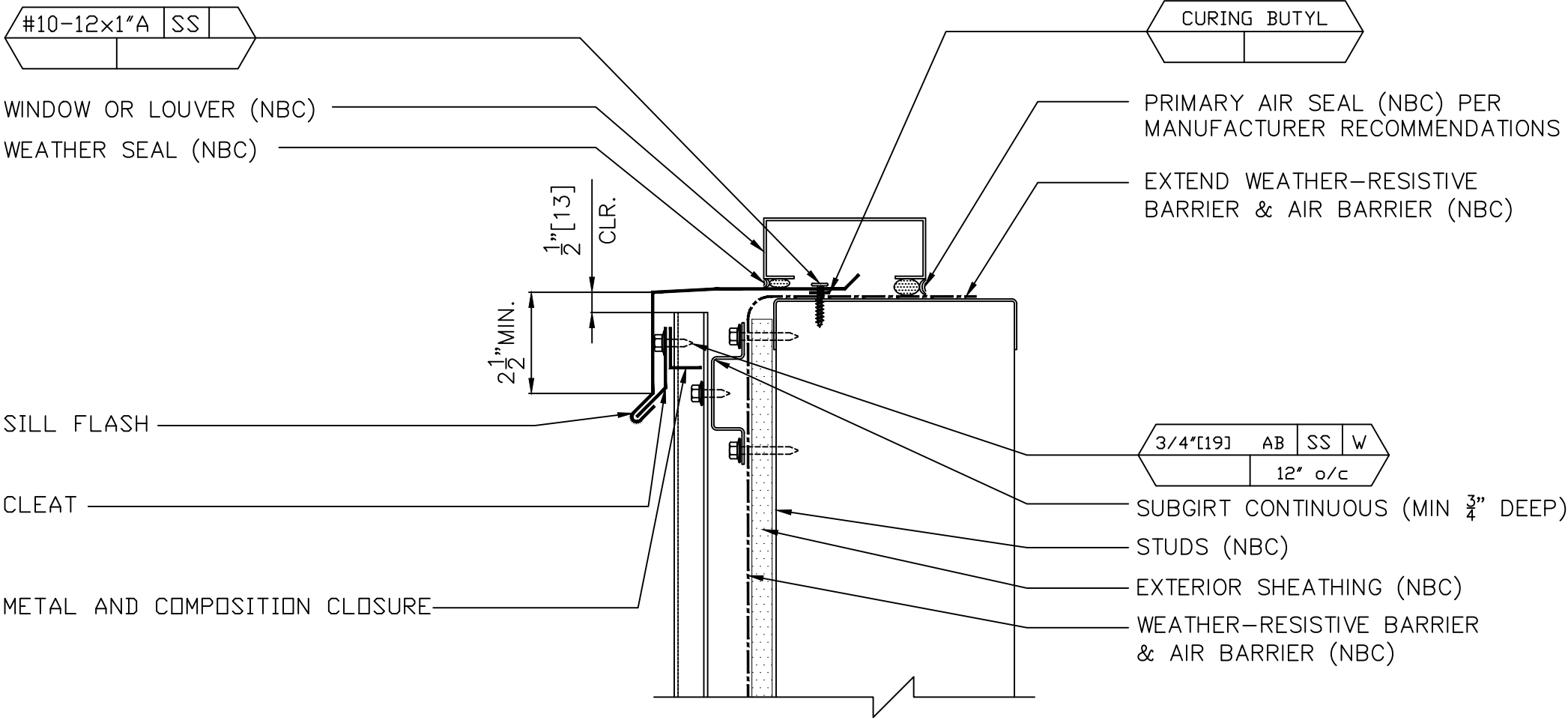
SILL OPENING (FLASHING)
