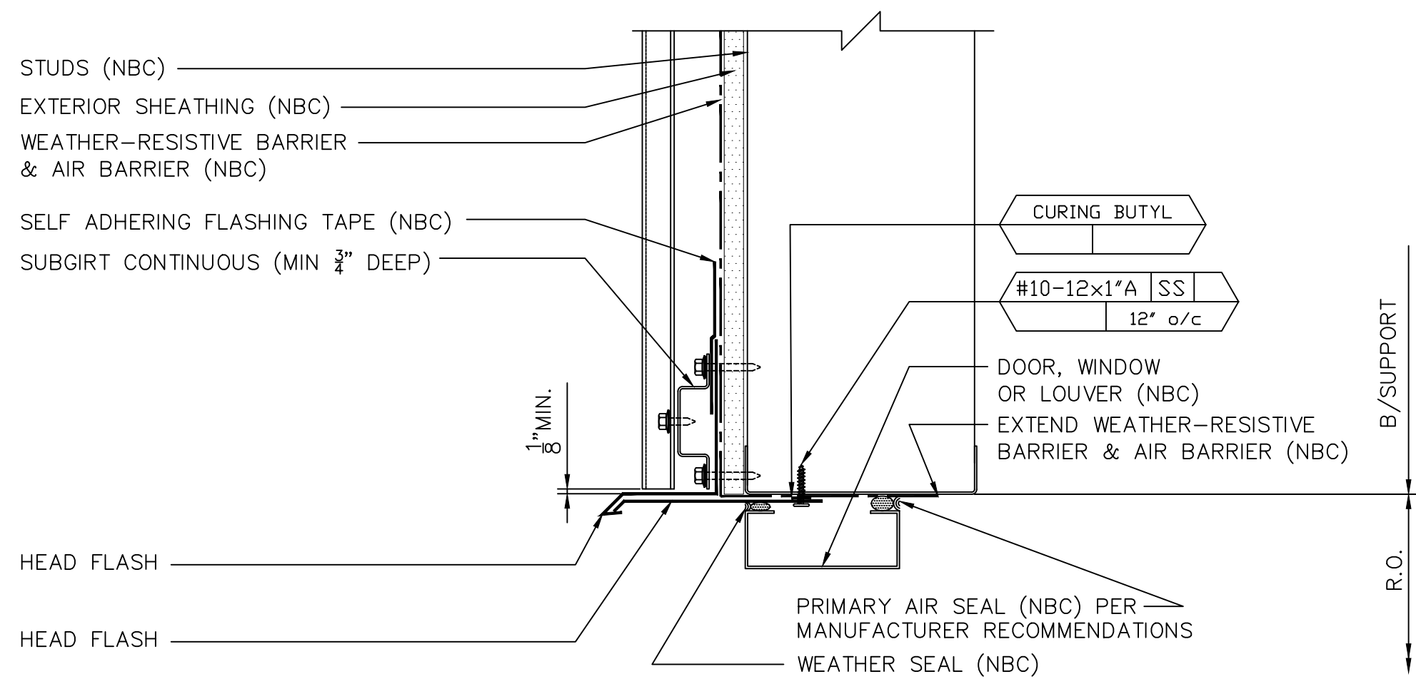
HEAD OPENING (FLASHING)
